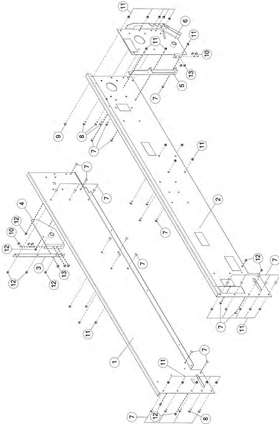
FIGURE 5 SIDE PANELS
